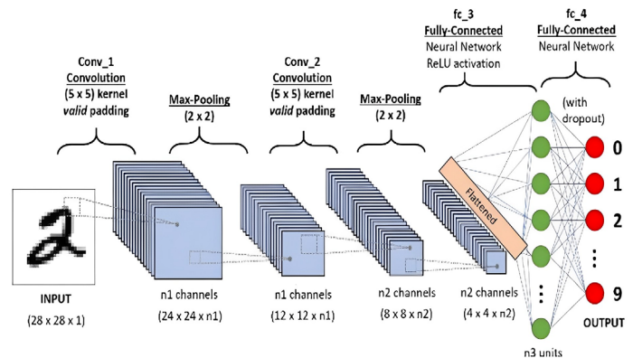
Figure 1. Convolutional Neural Network (CNN) Architecture
