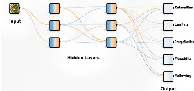
Figure 3. Neural Network
